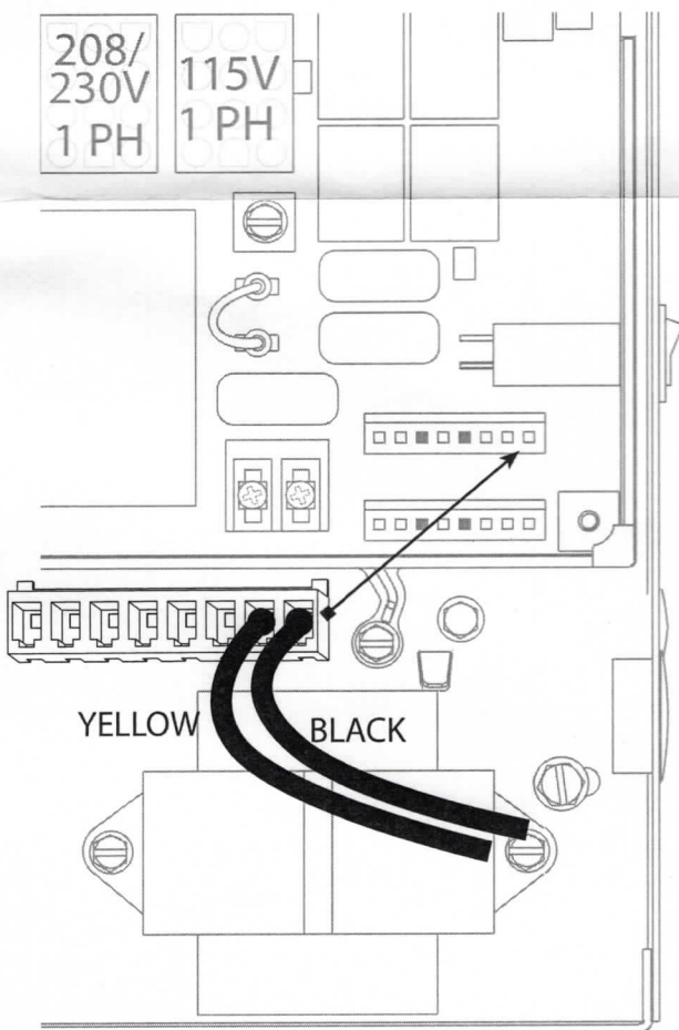
1 PHASE
