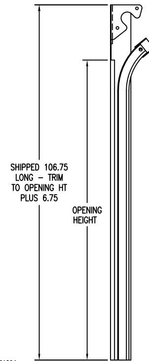
VERTICAL TRACK DETAIL
