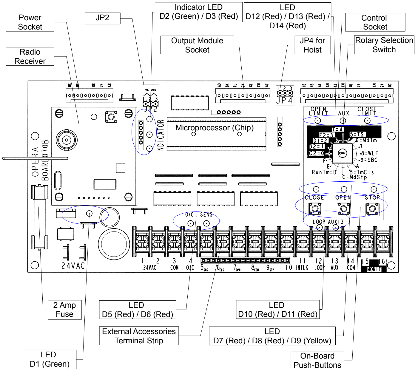
Figure 22 - Electronic Control Board – BOARD 070E
