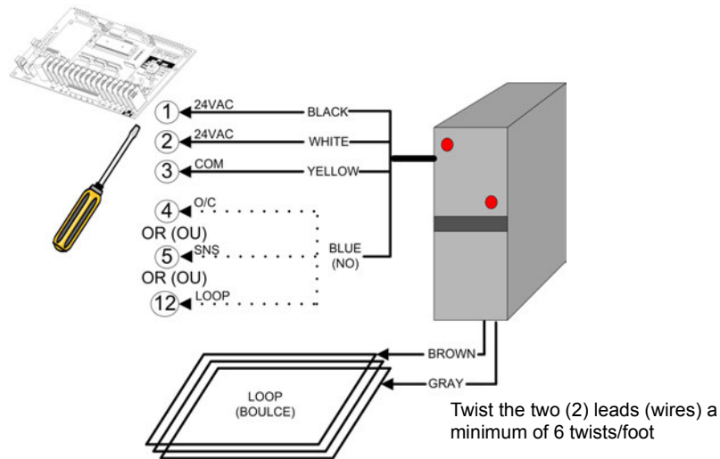
Figure 20 - Vehicle Loop Detector
