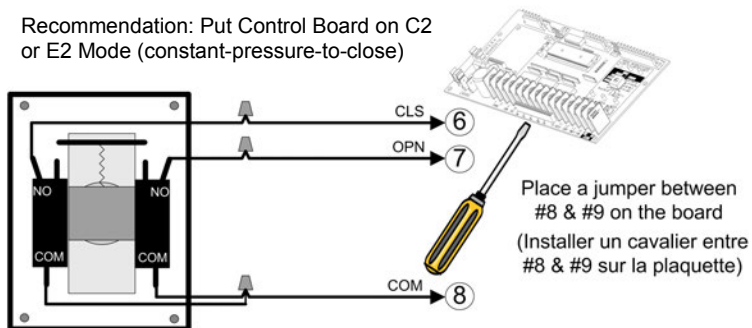
Figure 18 - KEYSWITCH 010 / 015
