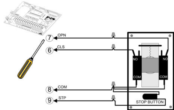
Figure 19 - KEYSWITCH 019
