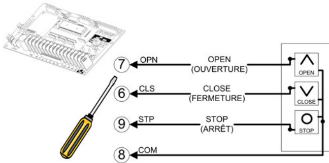
Figure 2 - STATION 020 / 084 3-PBS Open / Close / Stop
