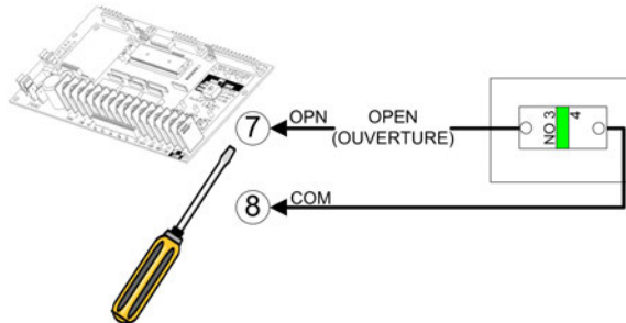
Figure 6 - STATION 001 / 081 1-PBS Open
