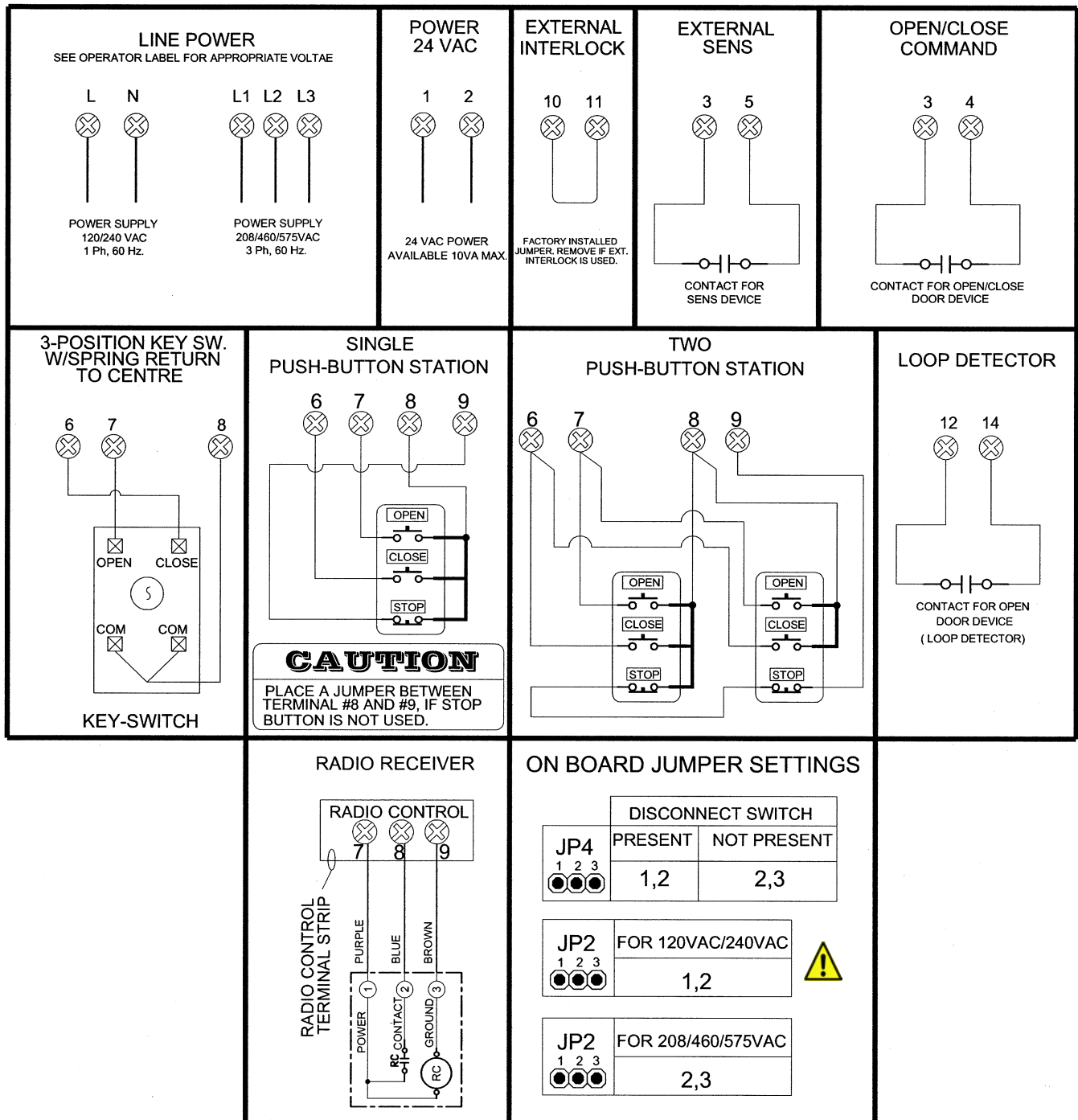
Figure 21 - External Wiring
