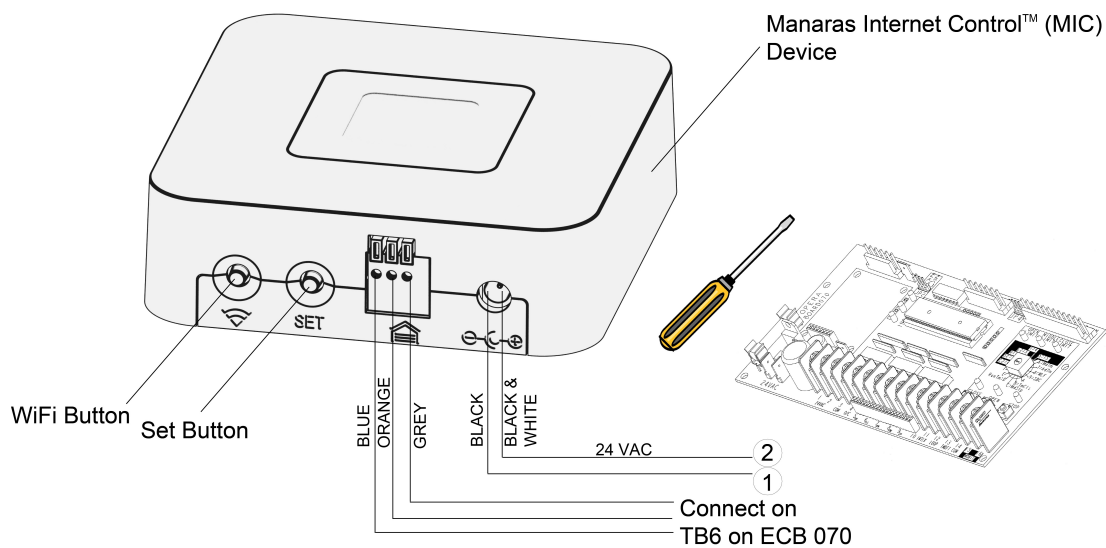
Figure 1 - Manaras Internet Control (MIC) Connection
