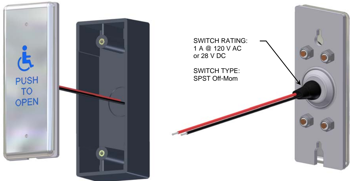
10PBJS1 Pushplate with Pushplate Box (pn 70.5054)
